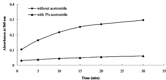
Figure 9. Effect of acetonitrile on the spectrophotometric signal intensity for NBT. Reactions were carried out at ambient temperature in PBS (100 mM, pH 7.4). All reaction mixtures contained 50 μL of 0.42 mM NBT, 50 μL of 5 mM H 2 O 2 , 50 μL of 5 mM EDTA, and 50 μL of 5 mM Fe 2+ in the absence (control: 5% PBS) or presence of 5% acetonitrile (v/v).
